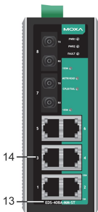
EDS-408A-MM-ST Front Panel View
