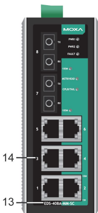
EDS-408A-MM-SC Front Panel View
