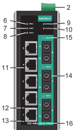
EDS-408A-3M-SC Front Panel View
