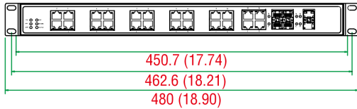
Front View
