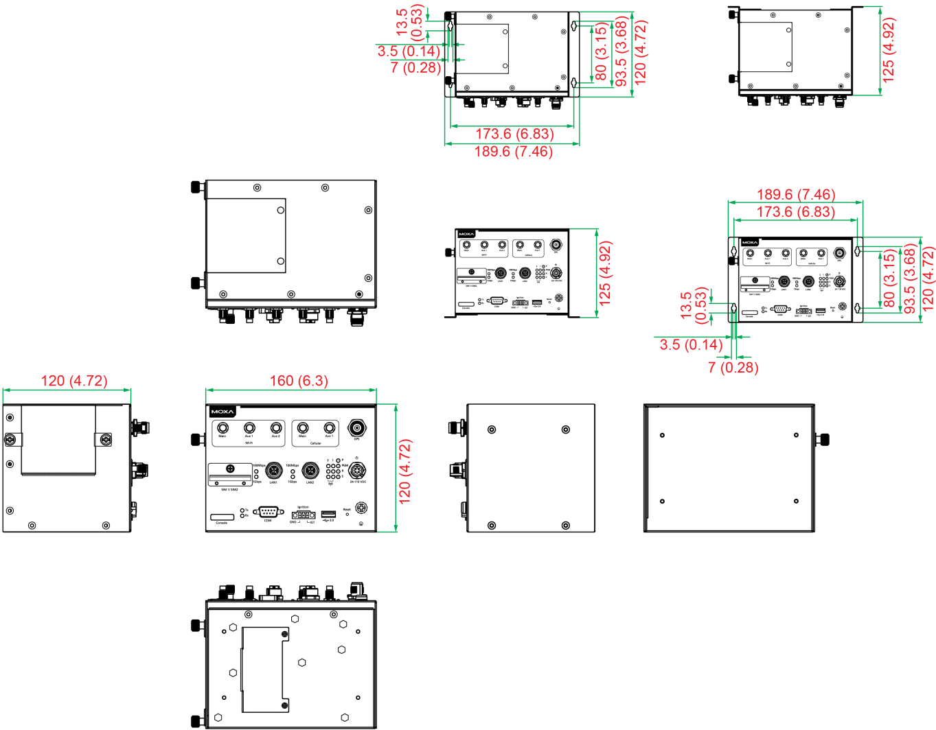
Mounting Type
