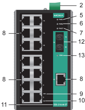
EDS-316-M-ST Front Panel View
