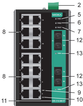
EDS-316-MM-ST Front Panel View
