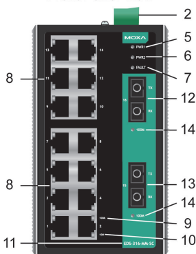
EDS-316-MM-SC Front Panel View
