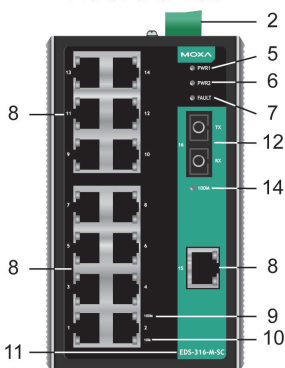
EDS-316-M-SC Front Panel View
