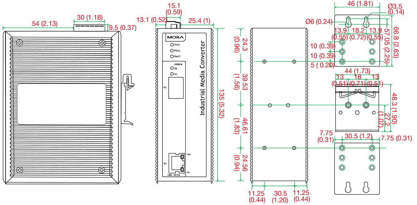
Side View
