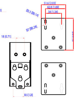
DIN-Rail/Panel Mount Kit
